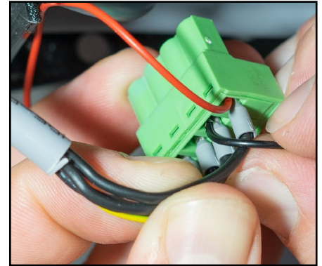
12. Loosen the two cables furthest from the yellow/black cable. Then insert the red cable from the fan unit in the utmost right edge position and the black cable next to it.
