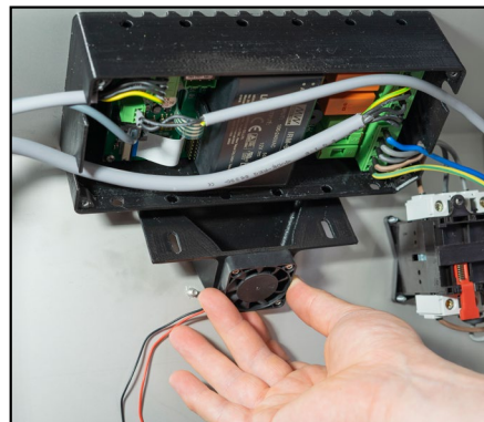
5. Hold the fan unit behind the black box, with the fan facing you and the screw holes facing upwards.
