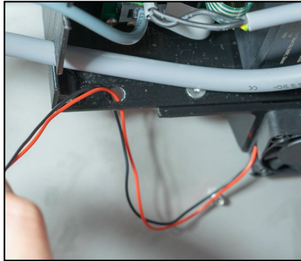
11. Lead the fan cables through the far left hole in the box, going in from the back.
