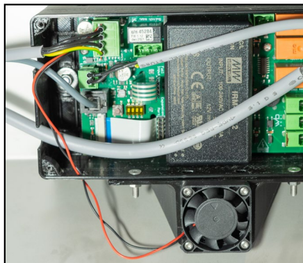
14. Refit the green plug onto the board.
