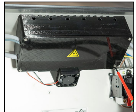
15. Screw the lid for the black box back on. Be careful not to over tighten. Turn on the machine briefly to verify the fan is running - then switch off the machine again.
