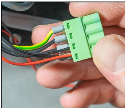
13. After inserting the cables from the fan unit, tighten the screws. The result should look like shown above.
