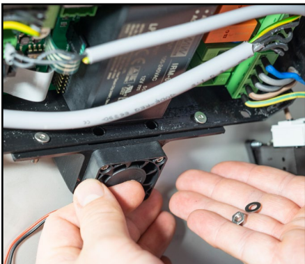
7. Put in the two screws. Place one screw at each corner. Ready the washers and nuts.
