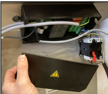
4. Remove the four screws and remove the lid from the black box.
