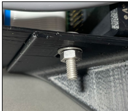
8. While pushing the fan unit backwards as much as possible, mount one washer and one nut for each screw. TAKE CARE NOT TO OVER TIGHTEN!
