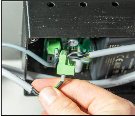
10. Pull out the green connector by yanking firmly. Make sure to pull it out straight, as the board pins may be damaged otherwise.
